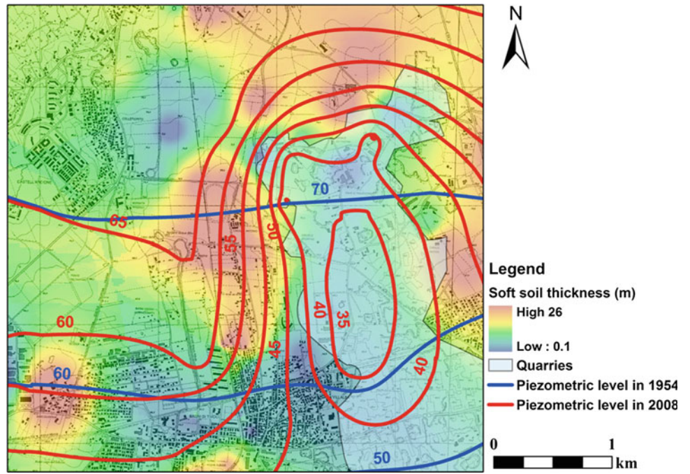
Fig. 31.2 Reconstruction via numerical modelling of piezometric levels within travertine in undisturbed (1954) and disturbed (2008) conditions superimposed on distribution of compressible soils thickness derived from boreholes log interpolation
