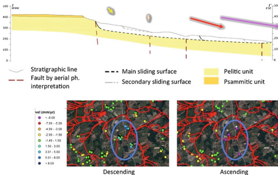
Fig. 35.3 Single landslide process dynamics derived combining ascending and descending A-DInSAR information. Vertical and horizontal displacement components have been inferred, so deriving the real displacement direction for all the landslide body portions
